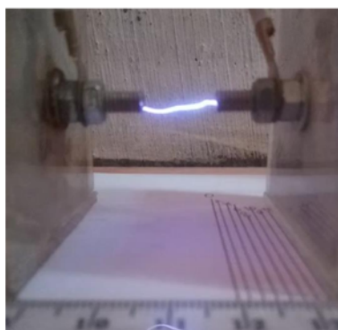
Figure 1. Spark jump test at a gap of 1.4 cm
