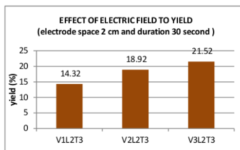
Figure 7. Effect of electric field strength to yield (L = 2 cm and for 30 second)
