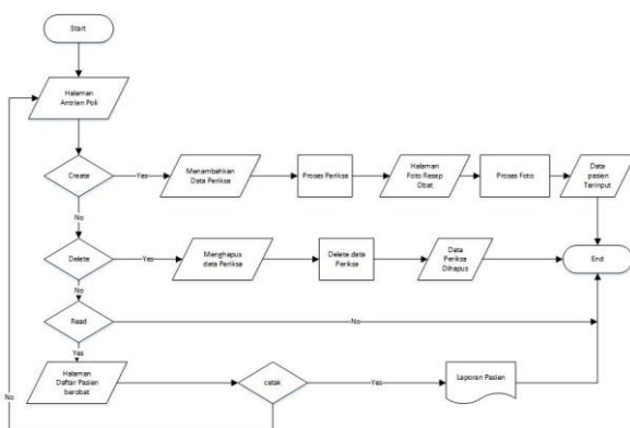
Gambar 7. Flowchart periksa
