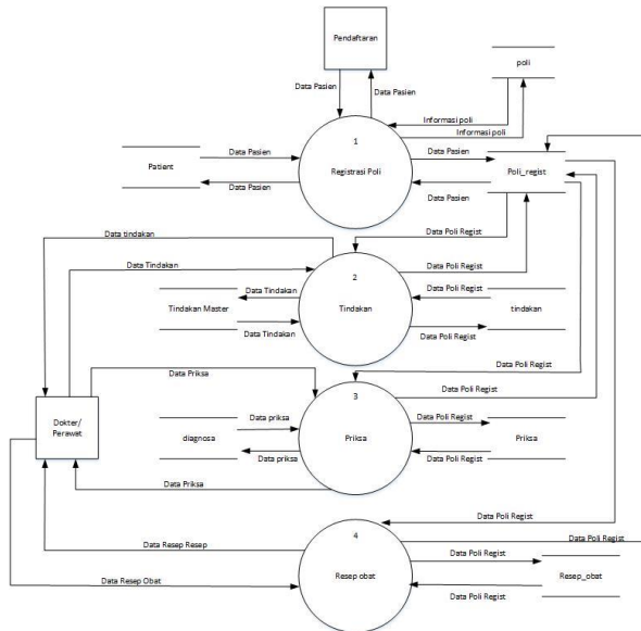
Gambar 4. DFD level 1
