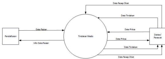
Gambar 3. DFD level 0
