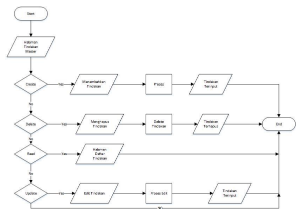
Gambar 9. Flowchart tindakan
