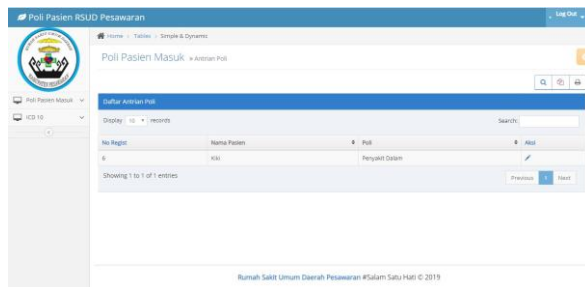
Gambar 11. Halaman Antrean
