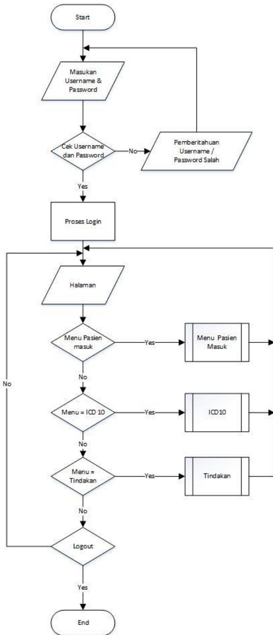
Gambar 6. Flowchart Authentication
